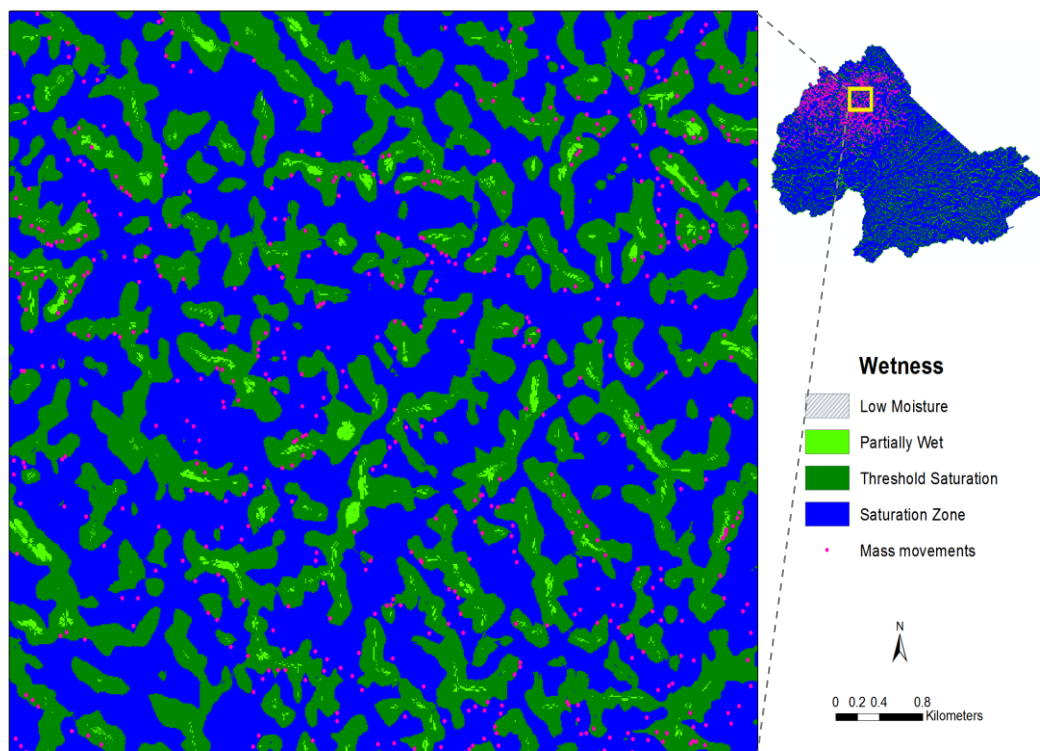
Figure 5. Wetness map.
