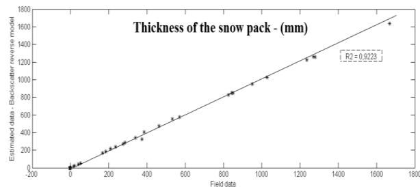
Fig. 2: linear regression between field data (snowpit) and modeled data.
