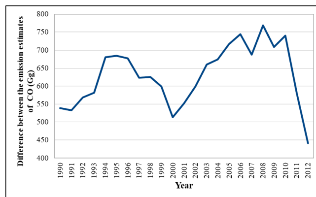
Figure 1. Difference between the CO emission estimates obtained using the SF proposed by Andreae and Merlet [3] and França et al. [4].
