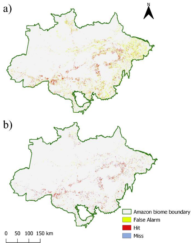
Figure 3. Deforestation data overlay map between a) PRODES and GFC; and b) PRODES and MapBiomass.
