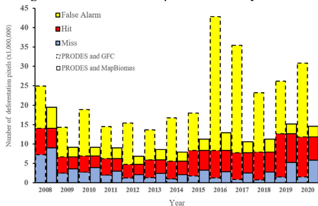
Figure 4. Number of Miss, Hit, and False Alarms pixels for each map pair.
