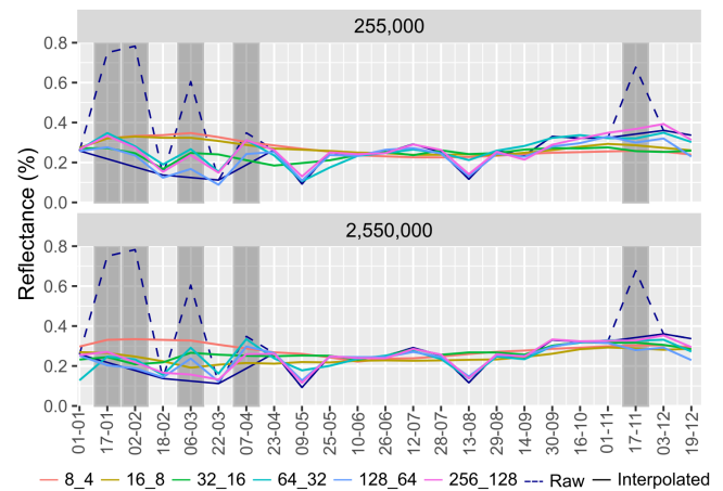
Figure 2: Result for the six models of each training set, comparing it to the linear interpolation and the raw data. The bars represent the cloud class extract from the SCL band.
