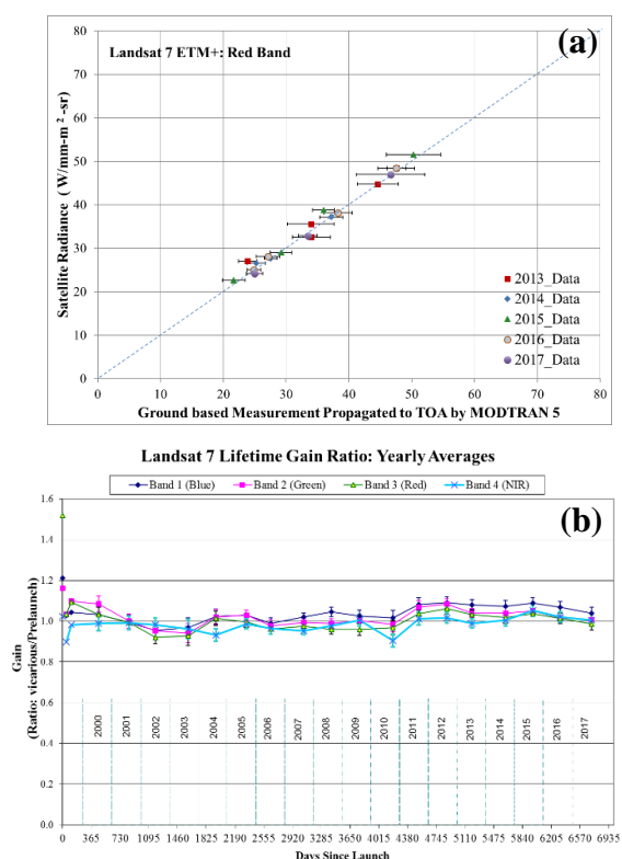
Figure 5. (a) Measured ETM+ Red band radiance versus MODTRAN-predicted surface radiance at SDSU site; (b) radiometric gain coefficient from 1999 to 2017 for ETM+ Blue, Green, Red and NIR spectral bands.
